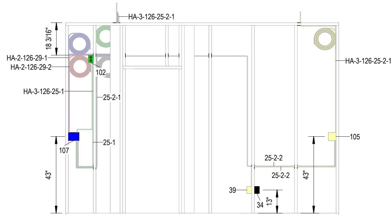
1 Electrical Side A 3/8" = 1'-0"
