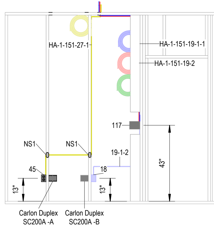
1 Electrical Side A 3/8" = 1'-0"
