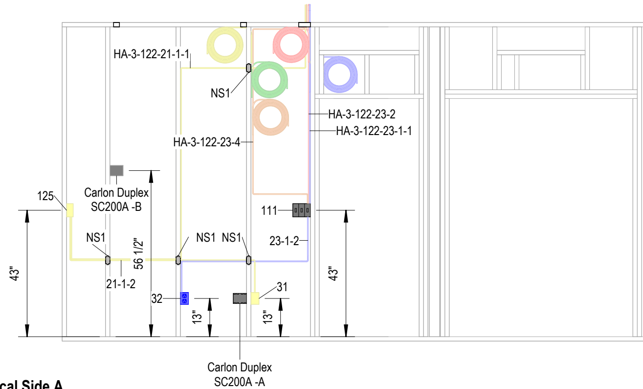
1 Electrical Side A 3/8" = 1'-0"
