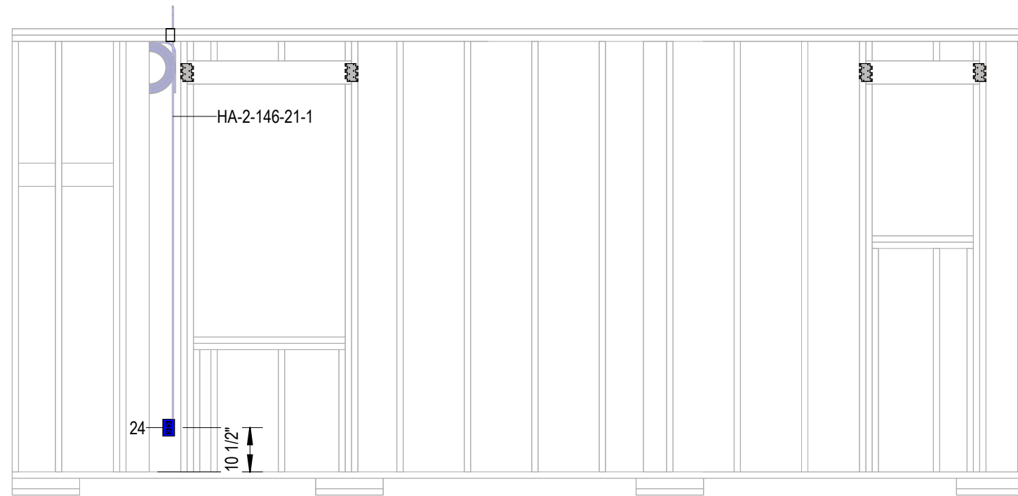
2 Electrical Side B 3/8" = 1'-0"
