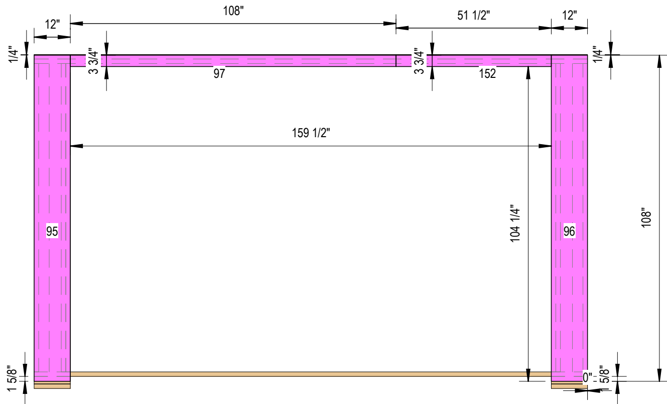
1 Sheathing Side A 3/8" = 1'-0"
