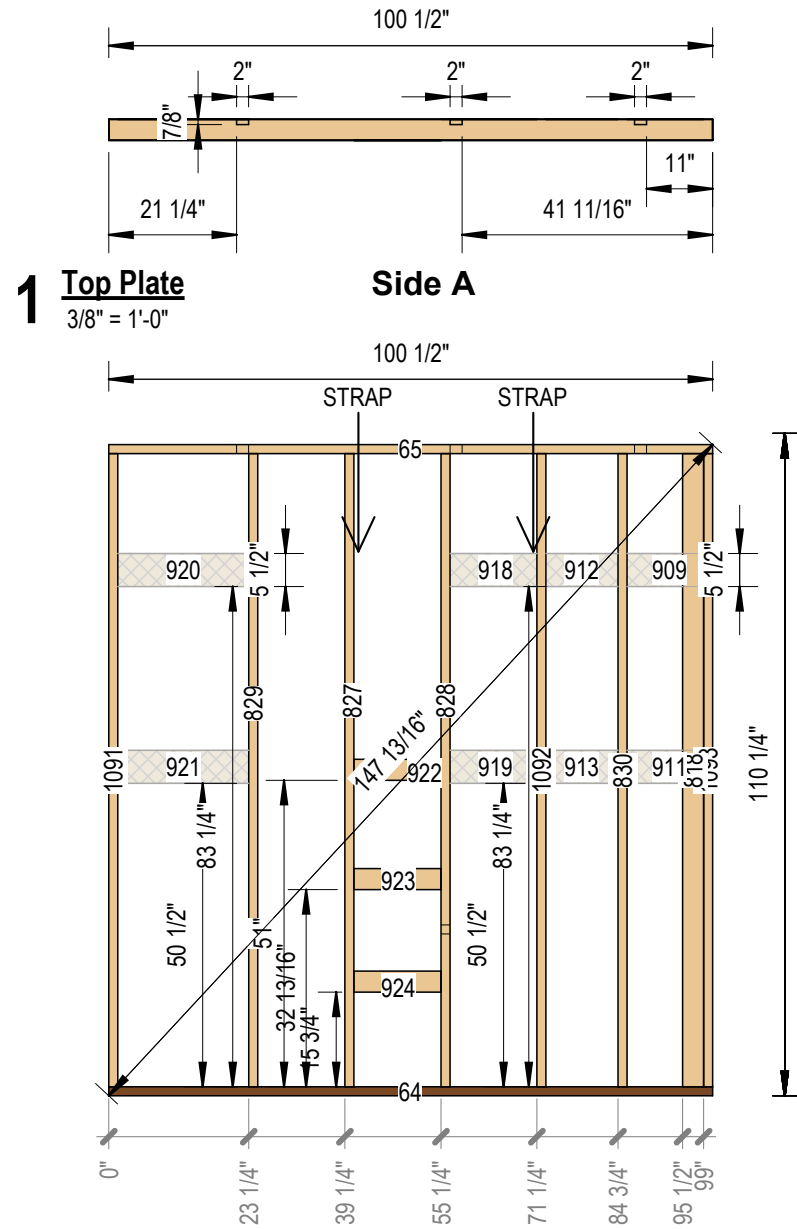
2 Framing Side A 3/8" = 1'-0"
