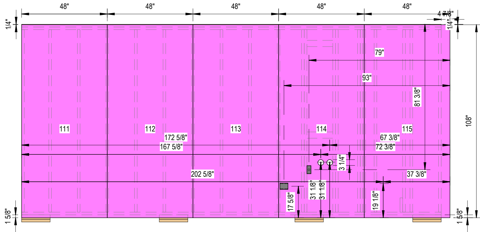
1 Sheathing Side A 3/8" = 1'-0"
