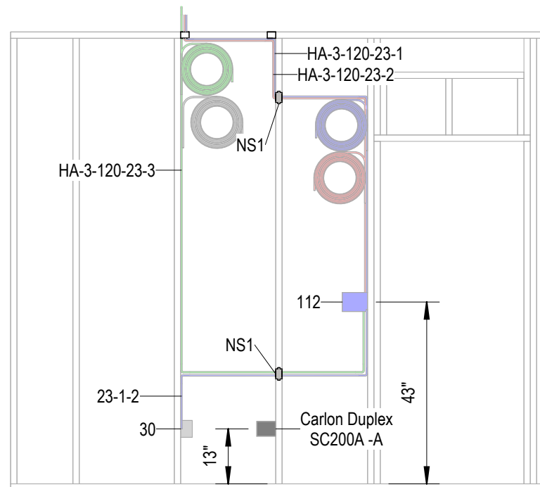
1 Electrical Side A 3/8" = 1'-0"
