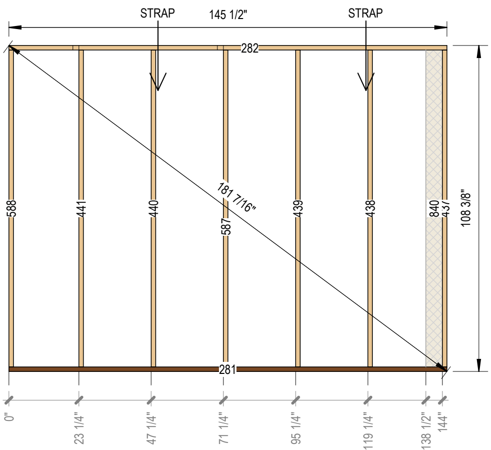
2 Framing Side A 3/8" = 1'-0"
