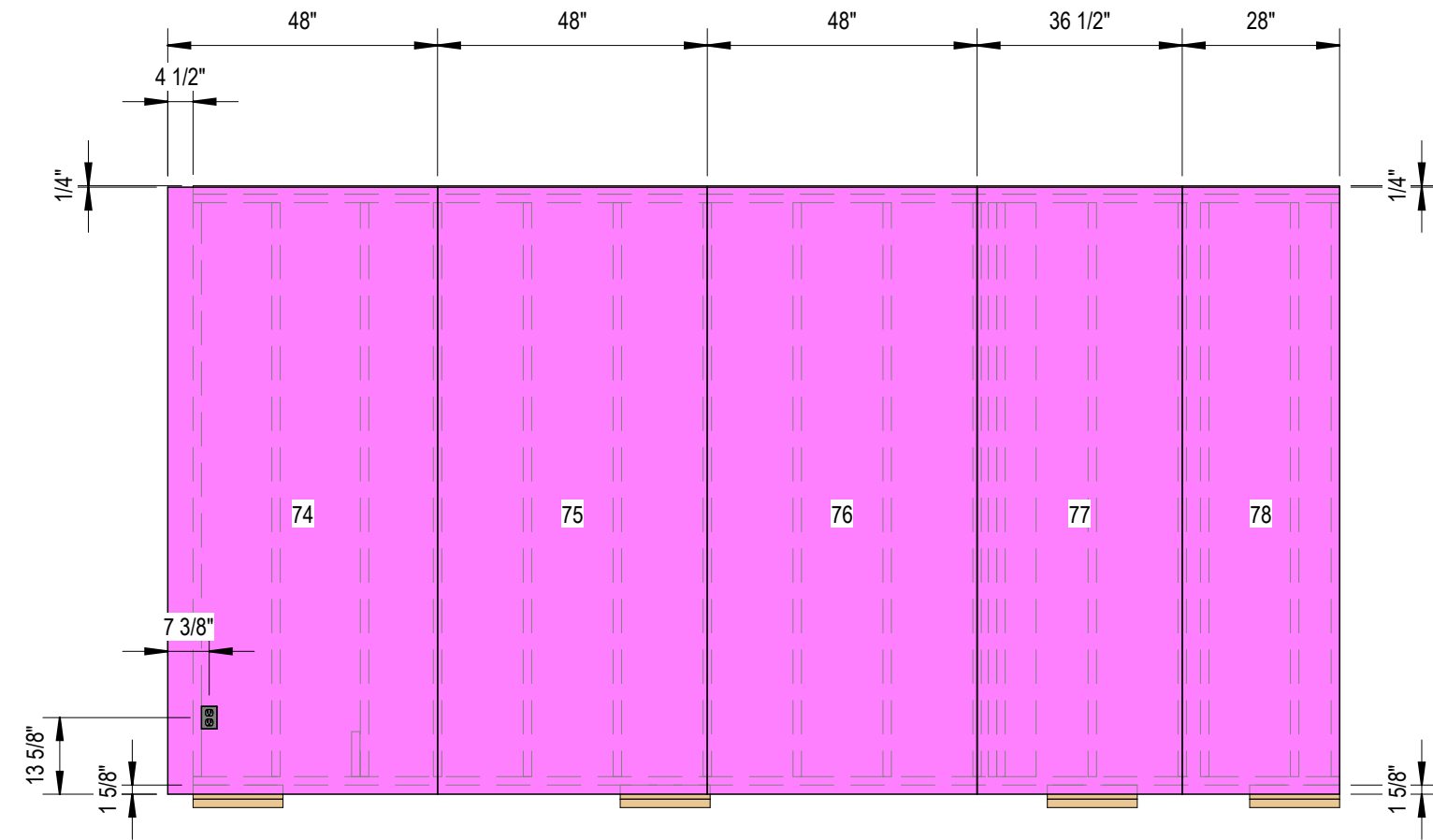
1 Sheathing Side A 3/8" = 1'-0"
