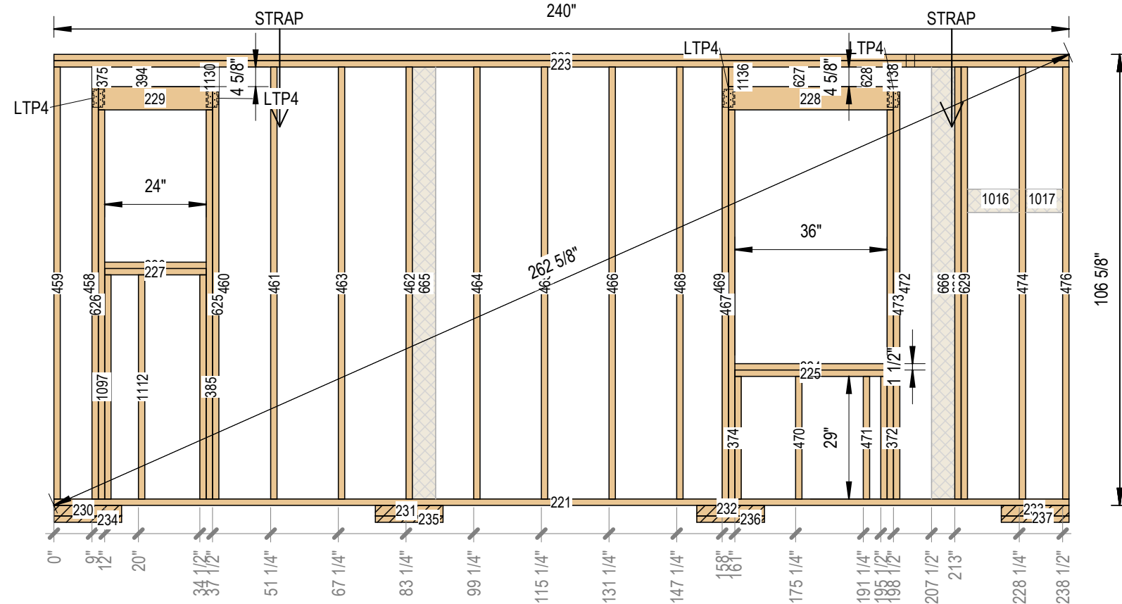
2 Framing Side A 3/8" = 1'-0"
