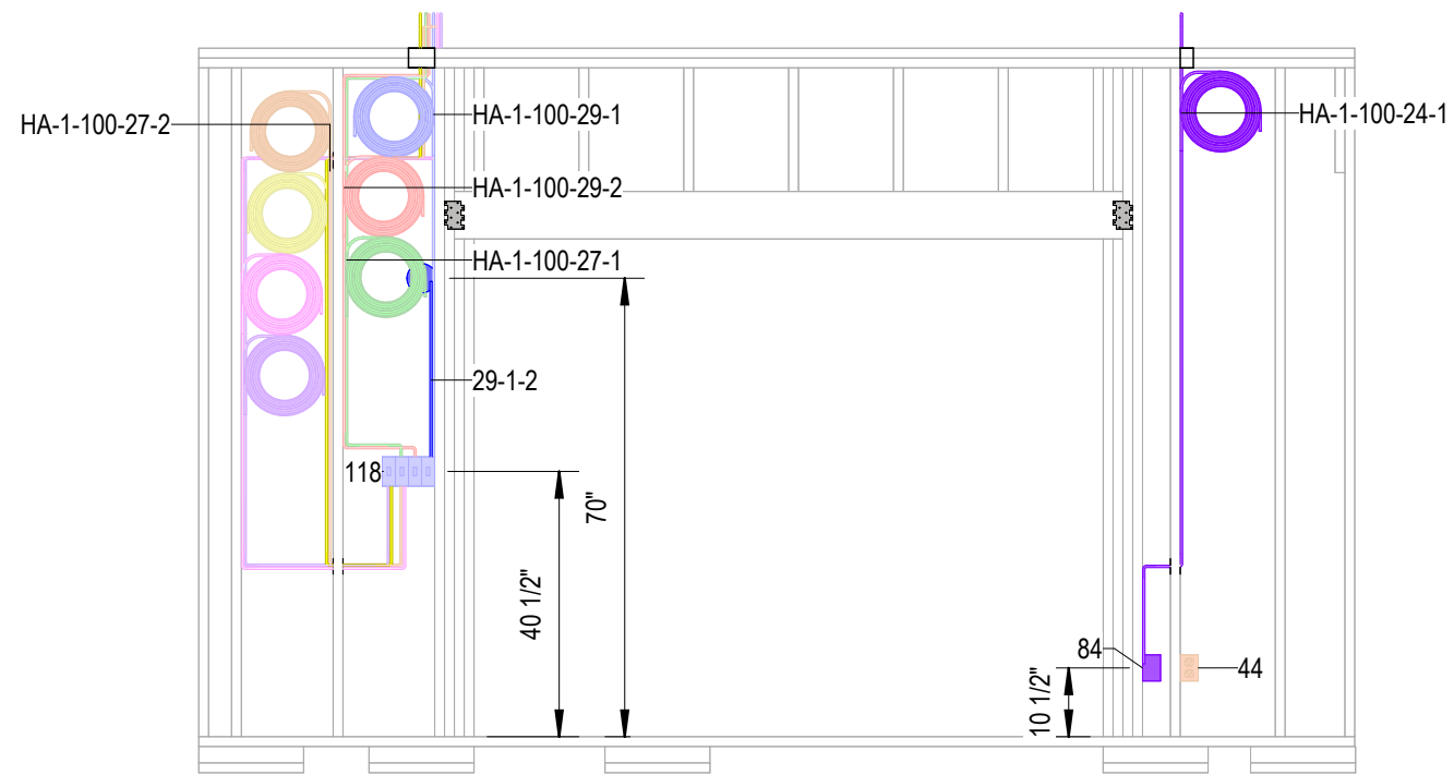
2 Electrical Side B 3/8" = 1'-0"
