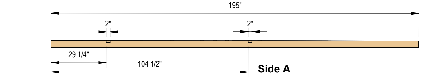
1 Top Plate 3/8" = 1'-0"
