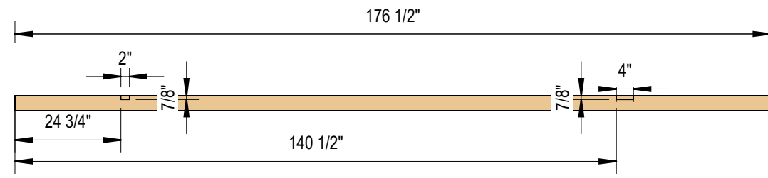
1 Top Plate 3/8" = 1'-0"
