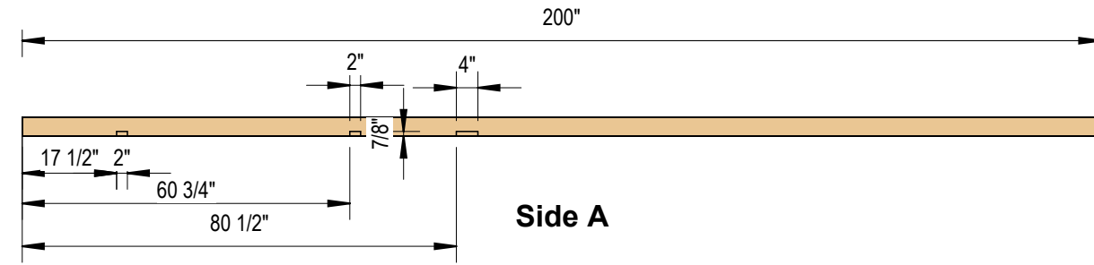
1 Top Plate 3/8" = 1'-0"
