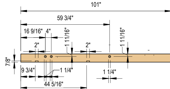
1 Top Plate 3/8" = 1'-0"
