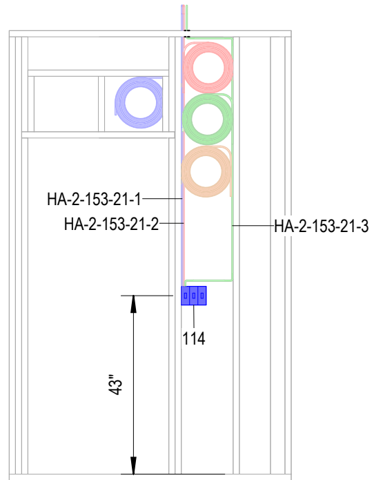
1 Electrical Side A 3/8" = 1'-0"
