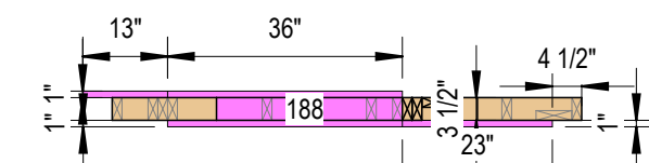
3 Sheathing Bottom View
