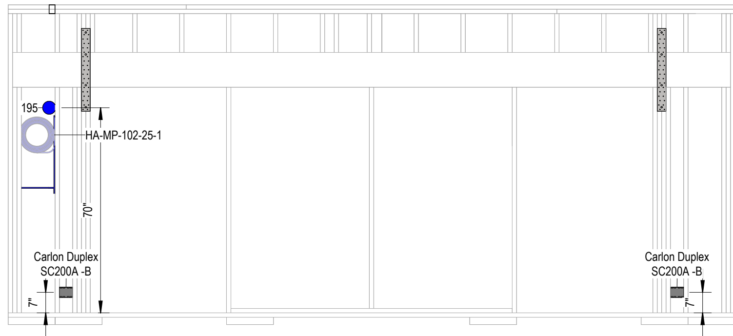
2 Electrical Side B 3/8" = 1'-0"
