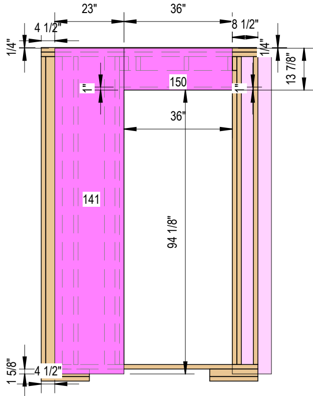
2 Sheathing Side B
