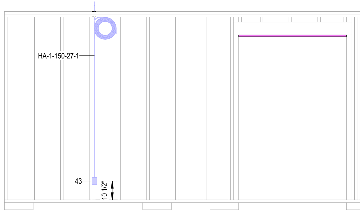
1 Electrical Side A 3/8" = 1'-0"
