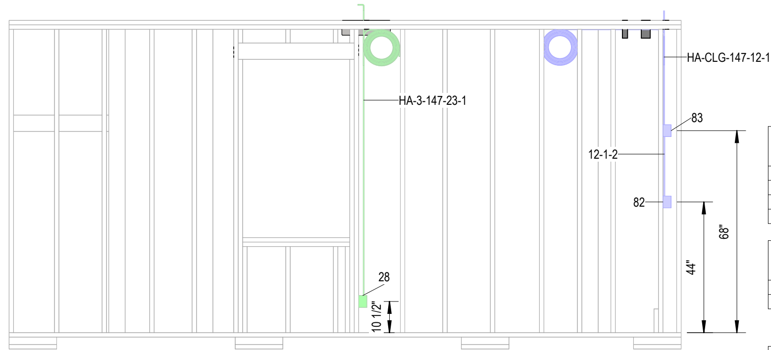
1 Electrical Elevation Side A 3/8" = 1'-0"
