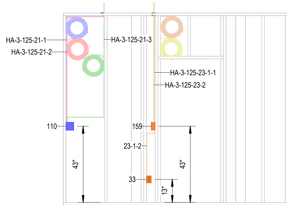
1 Electrical Side A 3/8" = 1'-0"
