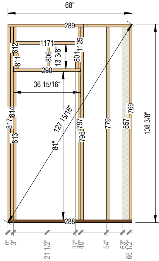
2 Framing Side A 3/8" = 1'-0"
