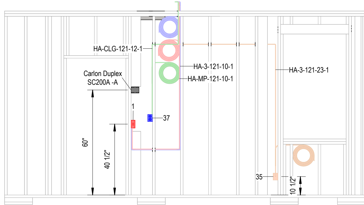
1 Electrical Side A 3/8" = 1'-0"
