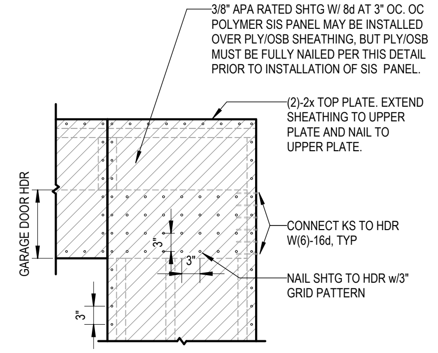
3 IRC PORTAL FRAME w/HDR (PFH) 3/4" = 1'-0"
