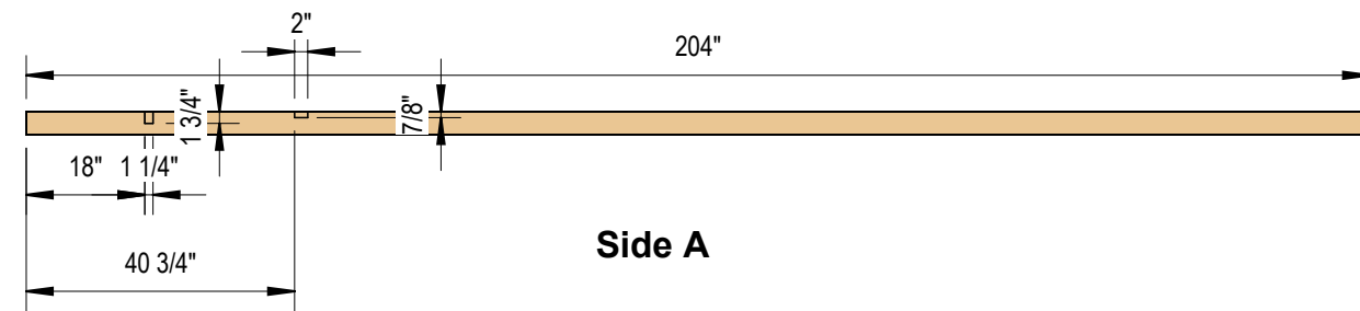
1 Top Plate 3/8" = 1'-0"
