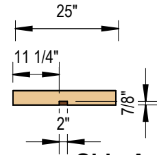
1 Top Plate 3/8" = 1'-0"
