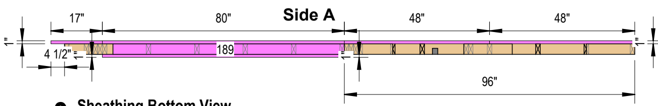
3 Sheathing Bottom View 3/8" = 1'-0"
