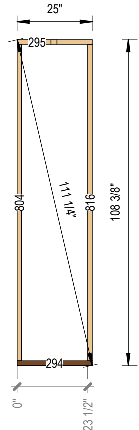
2 Framing Side A 3/8" = 1'-0"
