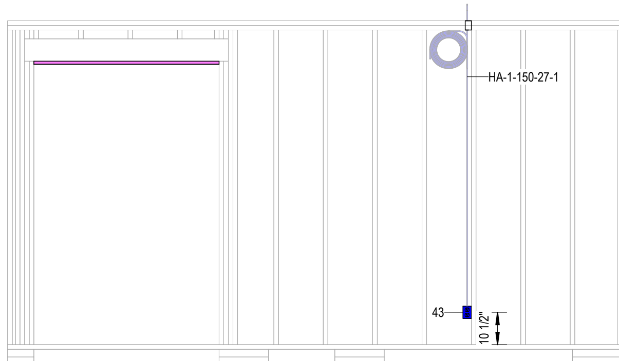
2 Electrical Side B 3/8" = 1'-0"
