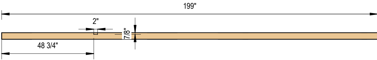
1 Top Plate 3/8" = 1'-0"
