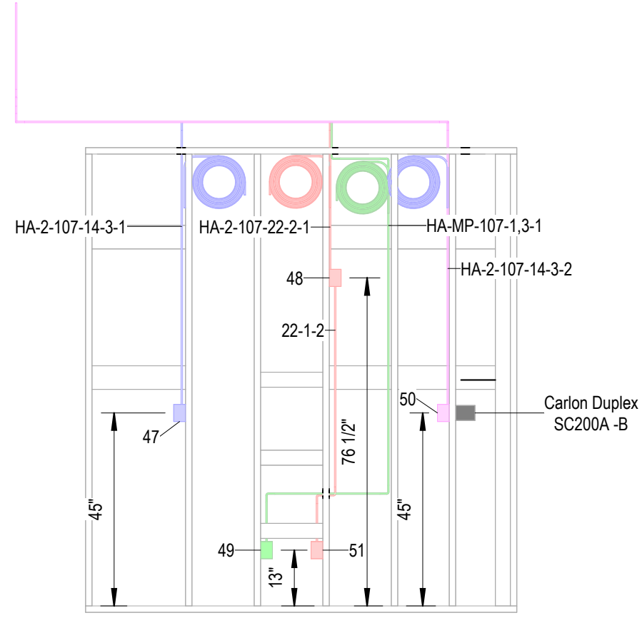
1 Electrical Side A 3/8" = 1'-0"
