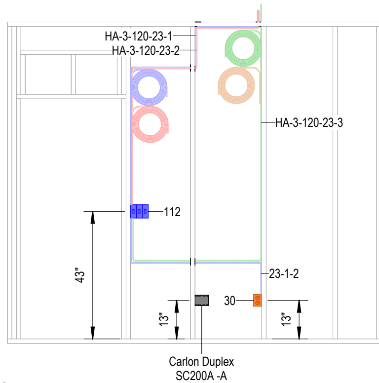
1 Electrical Side A 3/8" = 1'-0"
