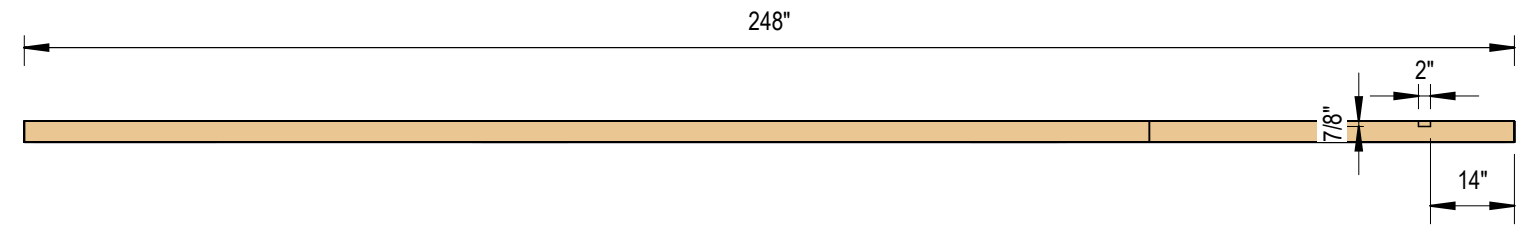
1 Top Plate 3/8" = 1'-0"
