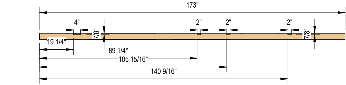
1 Top Plate 3/8" = 1'-0"
