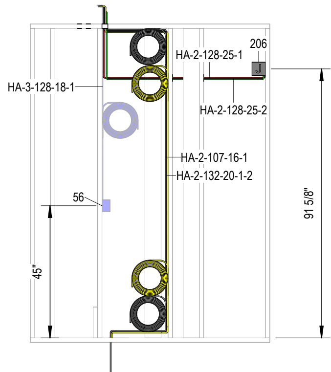
2 Electrical Side B 3/8" = 1'-0"
