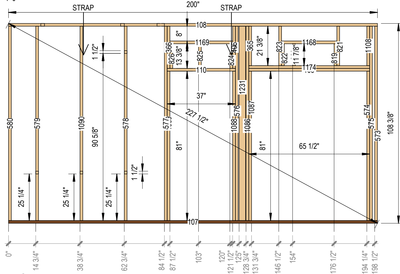
2 Framing Side A 3/8" = 1'-0"
