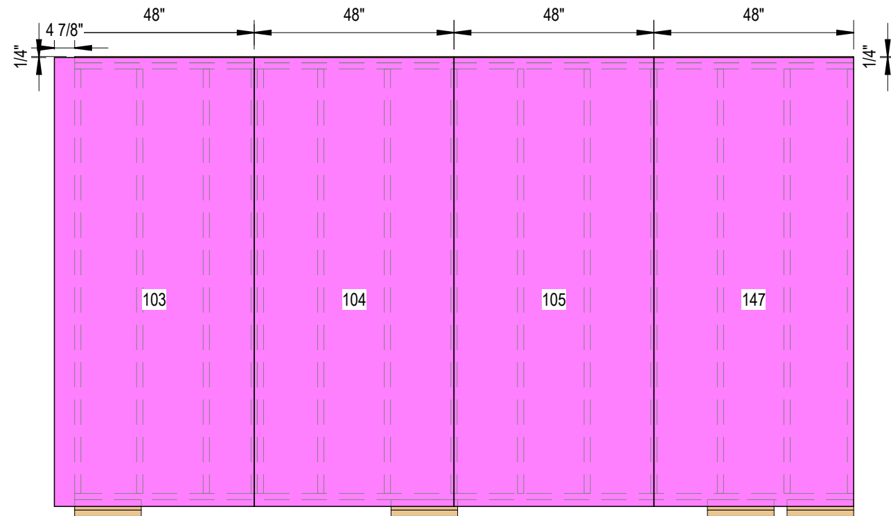
1 Sheathing Side A 3/8" = 1'-0"
