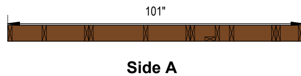
3 Bottom Plate 3/8" = 1'-0"
