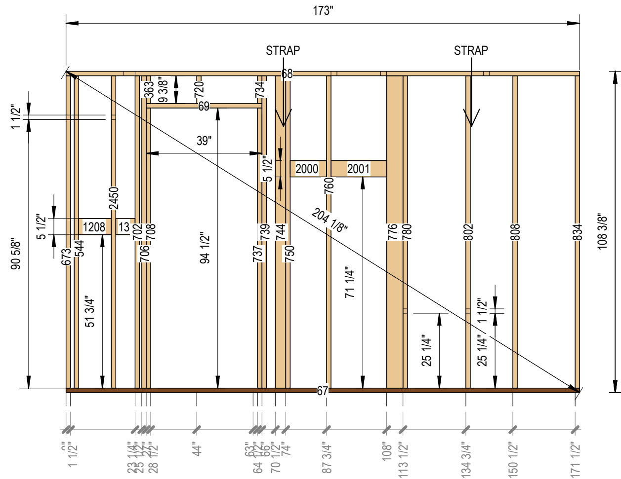
2 Framing Side A 3/8" = 1'-0"
