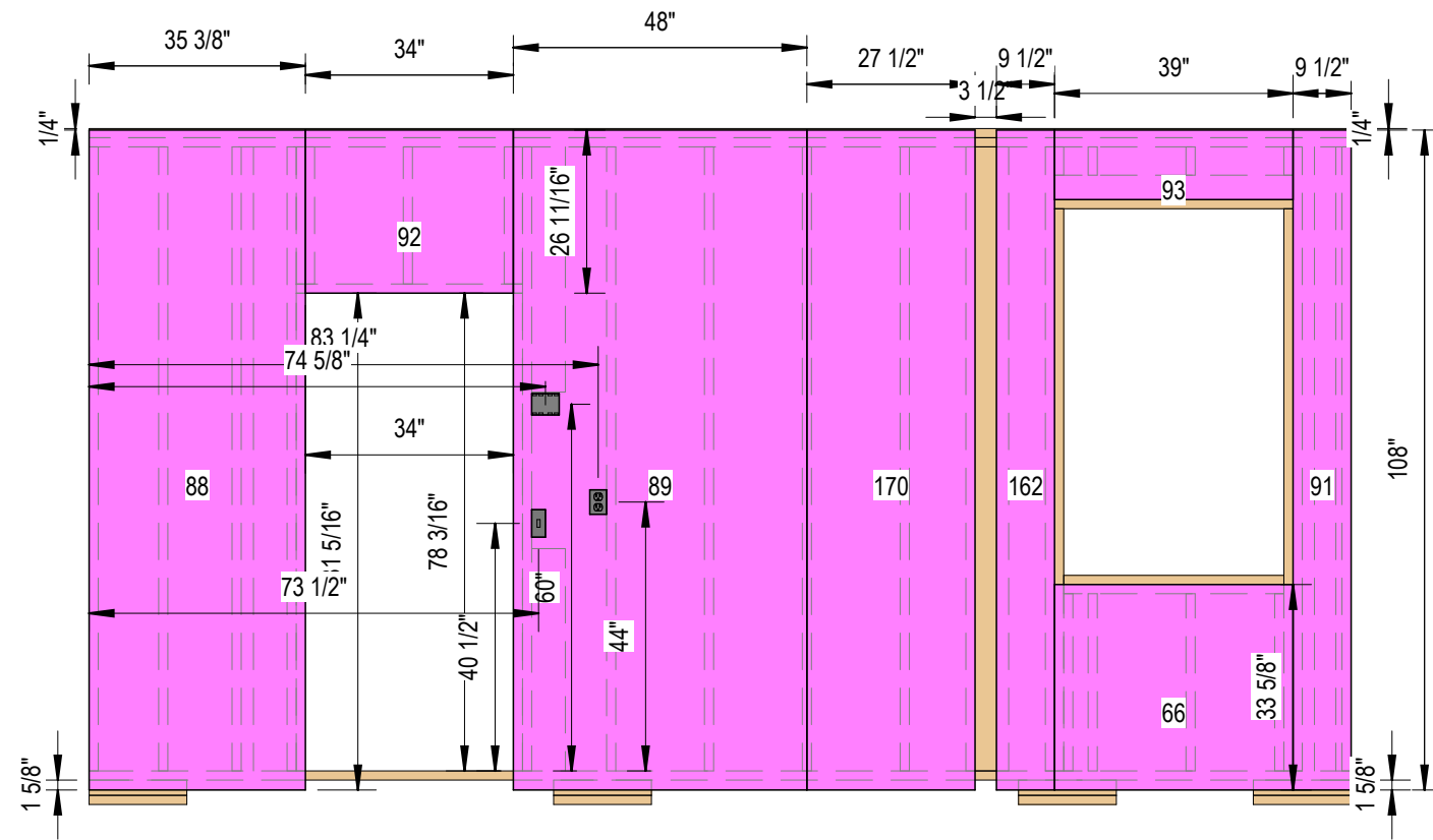
1 Sheathing Side A 3/8" = 1'-0"
