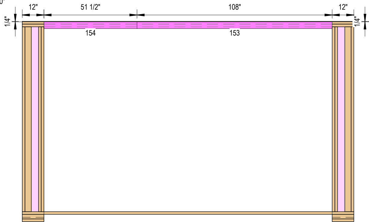
2 Sheathing Side B 3/8" = 1'-0"
