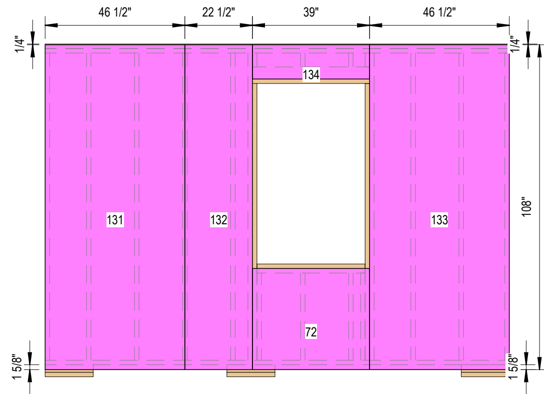
1 Sheathing Side A 3/8" = 1'-0"
