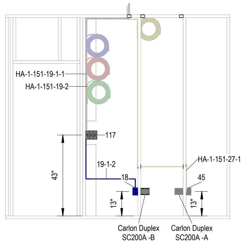
2 Electrical Side B 3/8" = 1'-0"
