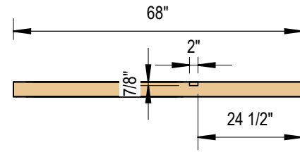
1 Top Plate 3/8" = 1'-0"
