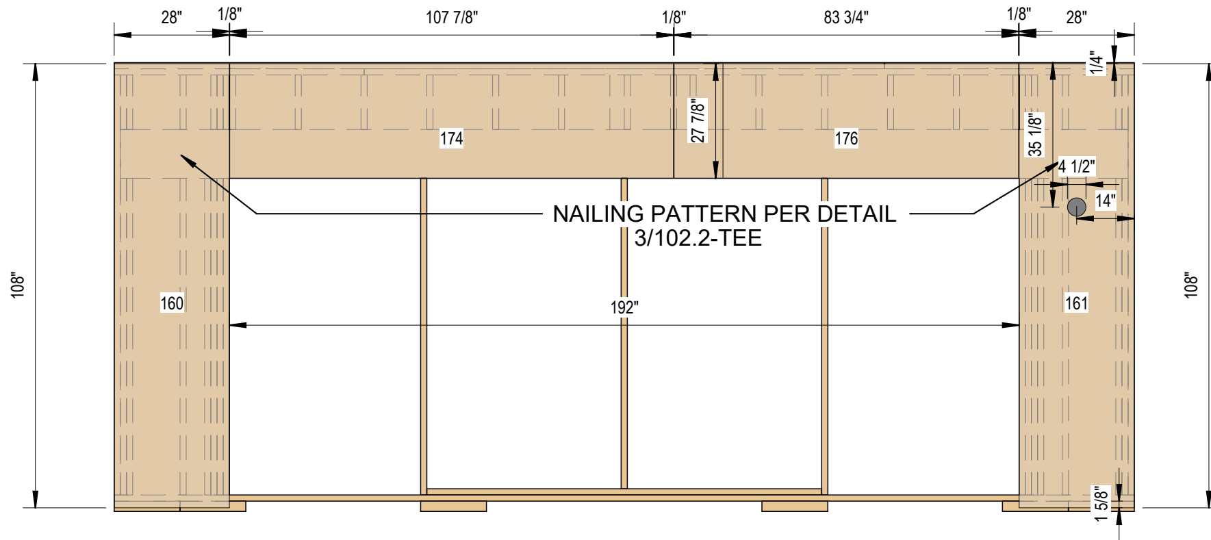
1 Sheathing OSB Side A 3/8" = 1'-0"
