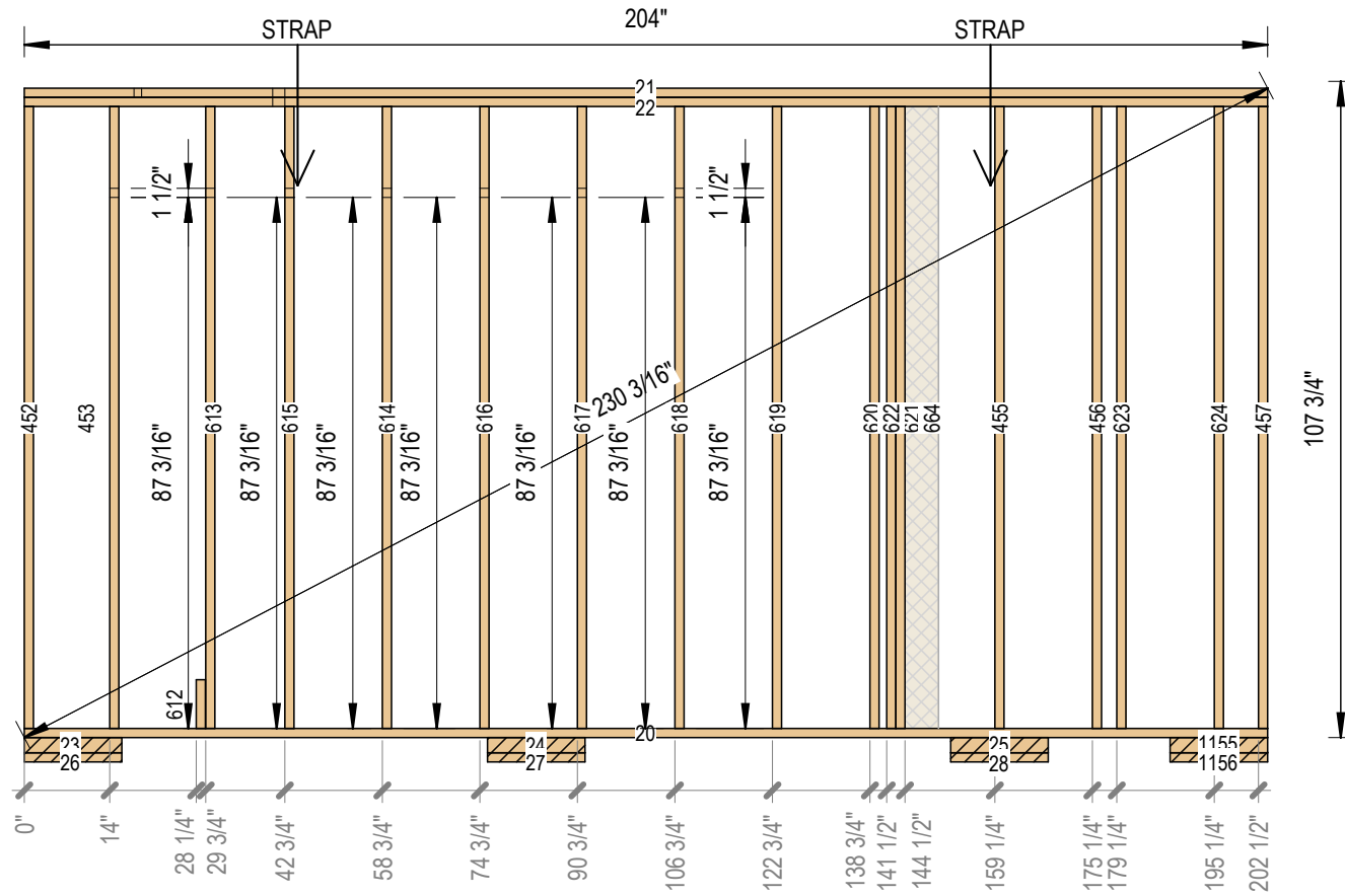
2 Framing Side A 3/8" = 1'-0"
