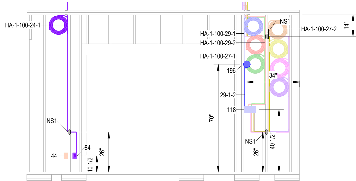
1 Electrical Side A 3/8" = 1'-0"
