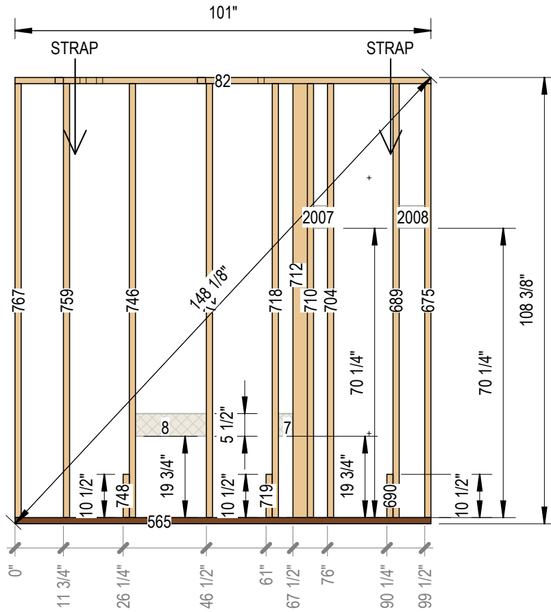
2 Framing Side A 3/8" = 1'-0"
