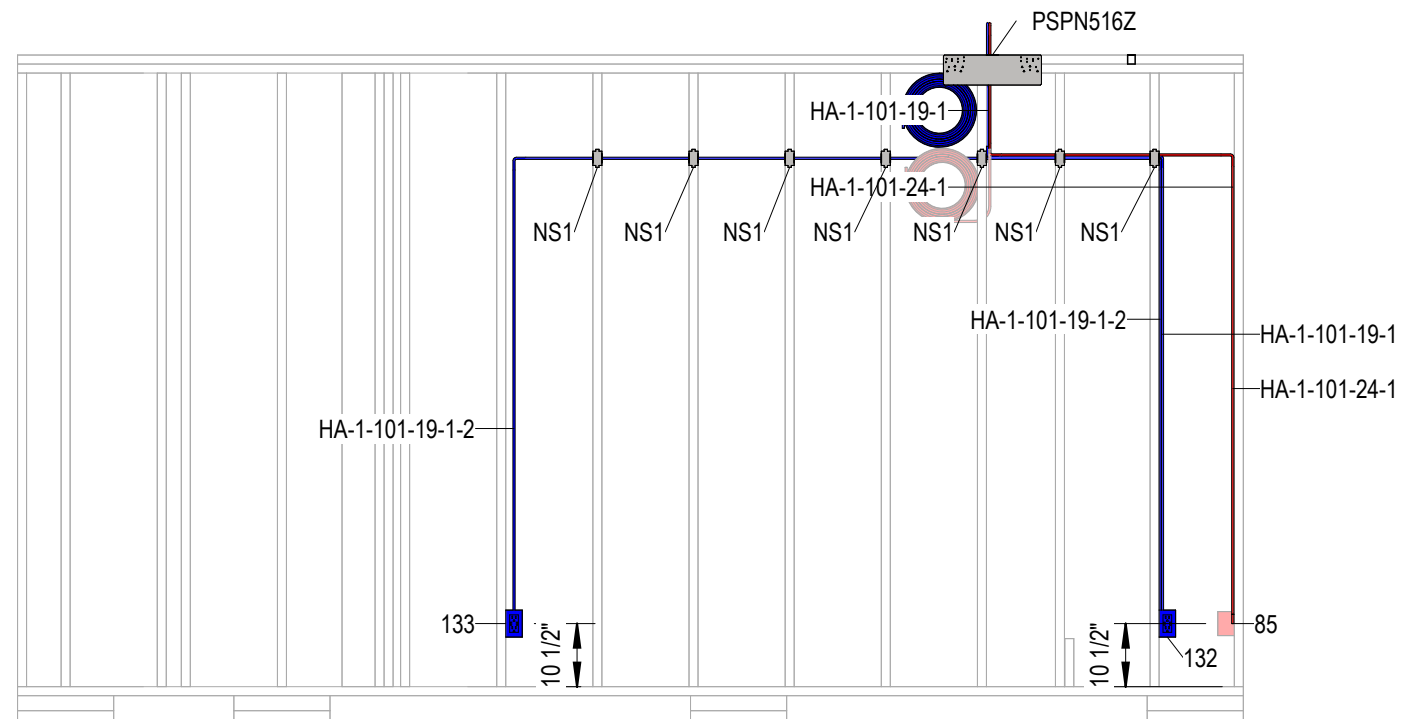
2 Electrical Side B 3/8" = 1'-0"
