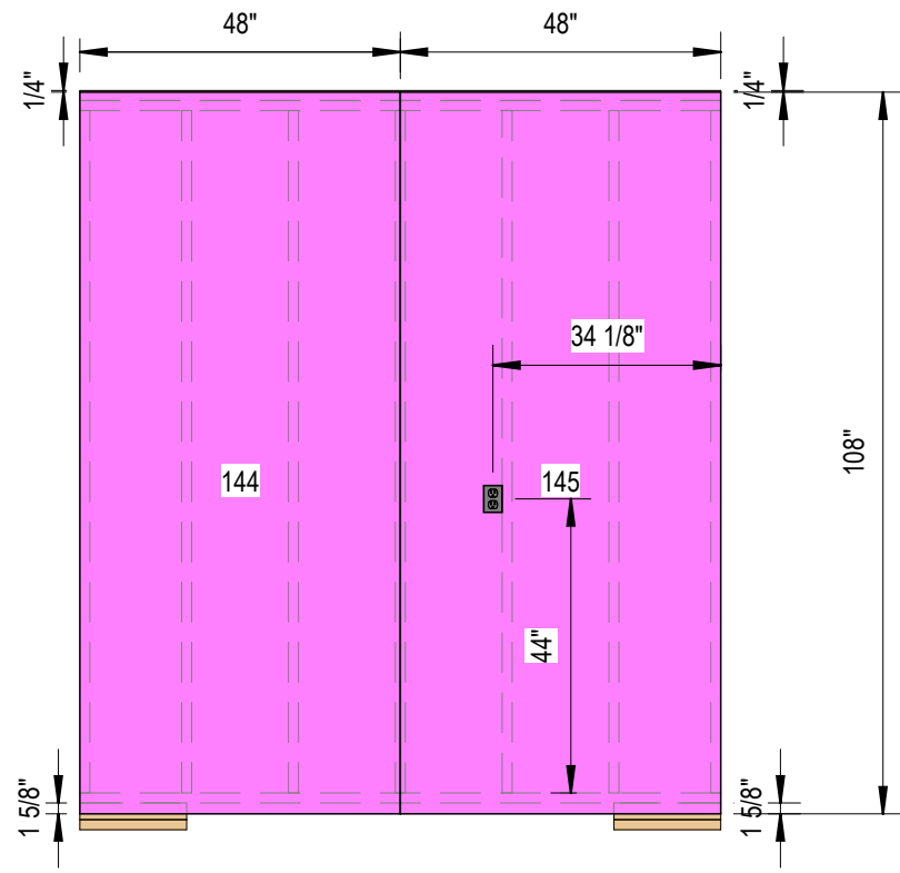
1 Sheathing Side A 3/8" = 1'-0"
