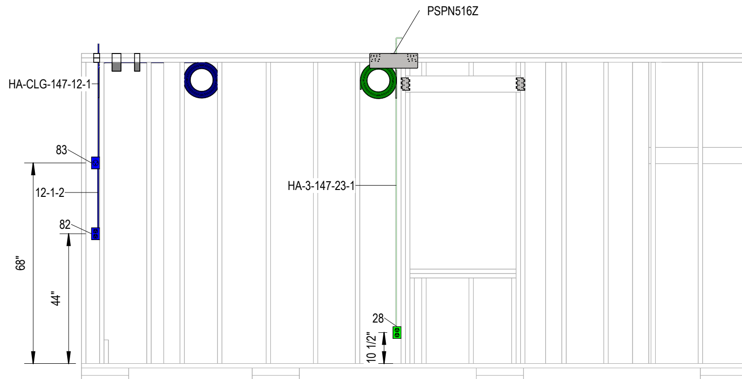
1 Electrical Elevation Side A 3/8" = 1'-0"
