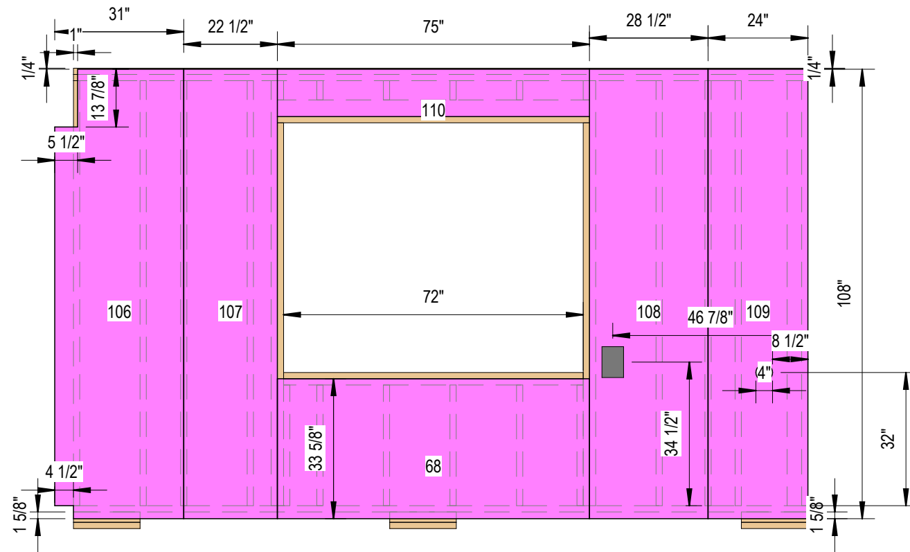
1 Sheathing Side A 3/8" = 1'-0"
