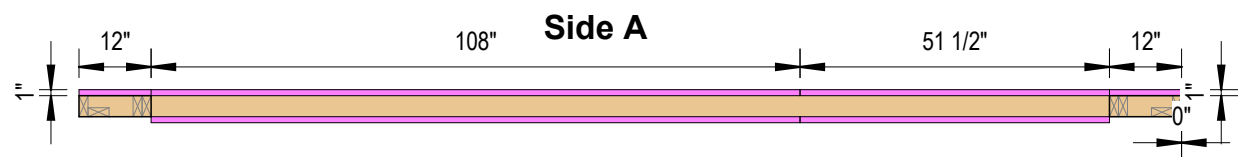
3 Sheathing Bottom View 3/8" = 1'-0"
