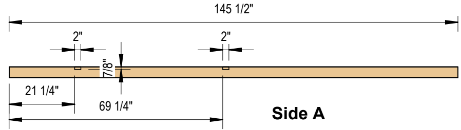
1 Top Plate 3/8" = 1'-0"
