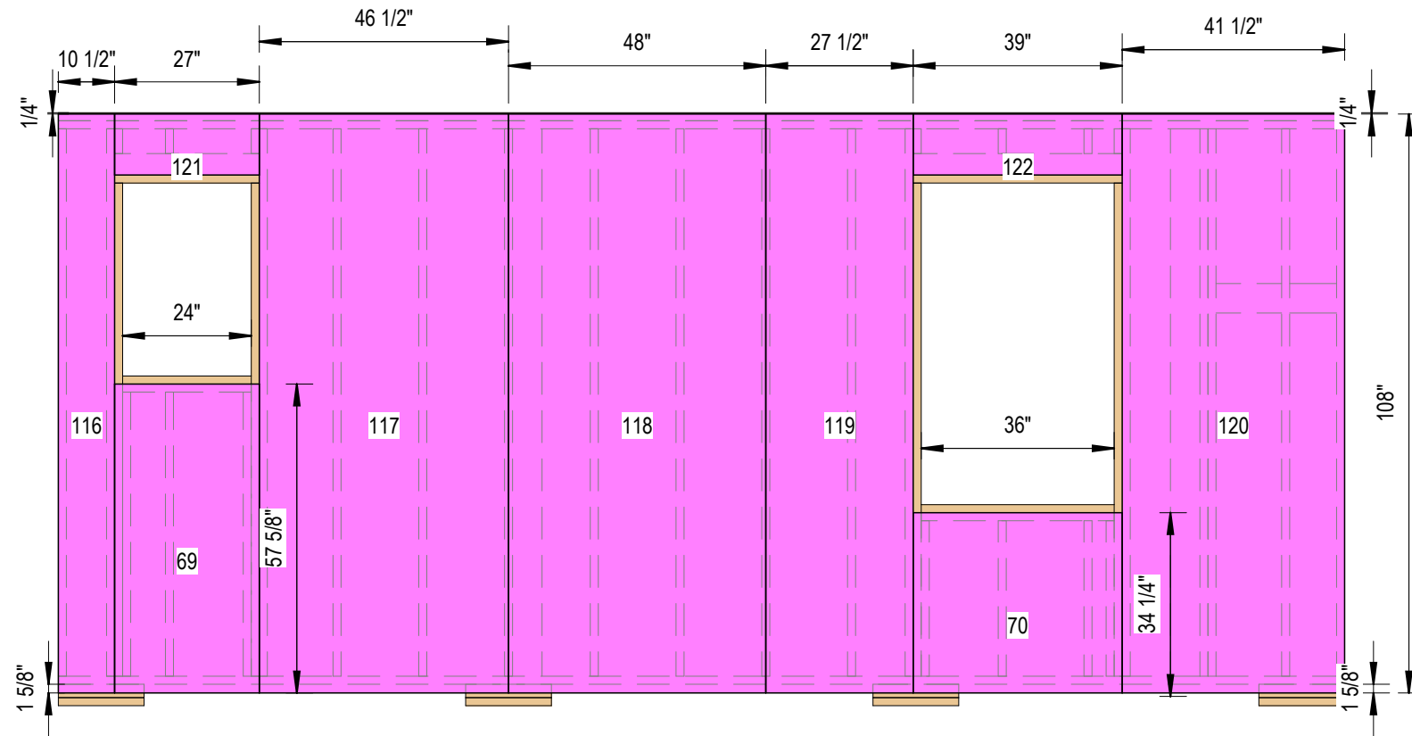
1 Sheathing Side A 3/8" = 1'-0"
