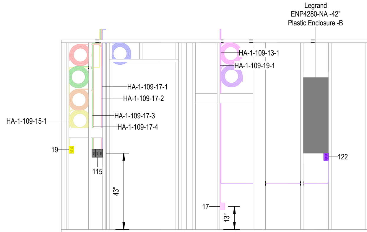
1 Electrical Side A 3/8" = 1'-0"
