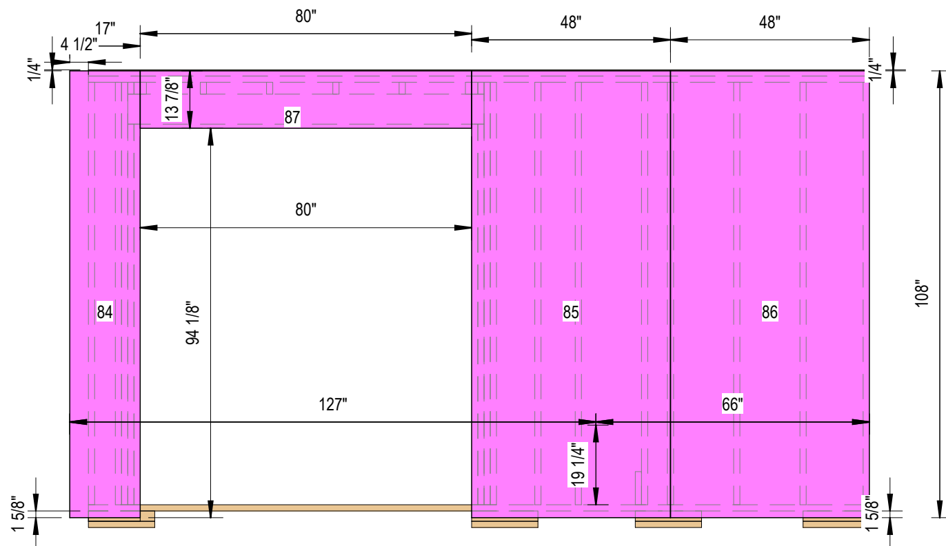
1 Sheathing Side A 3/8" = 1'-0"
