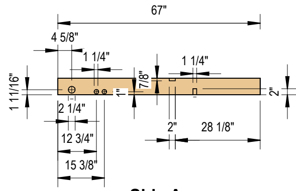
1 Top Plate 3/8" = 1'-0"
