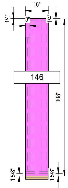
1 Sheathing Side A 3/8" = 1'-0"
