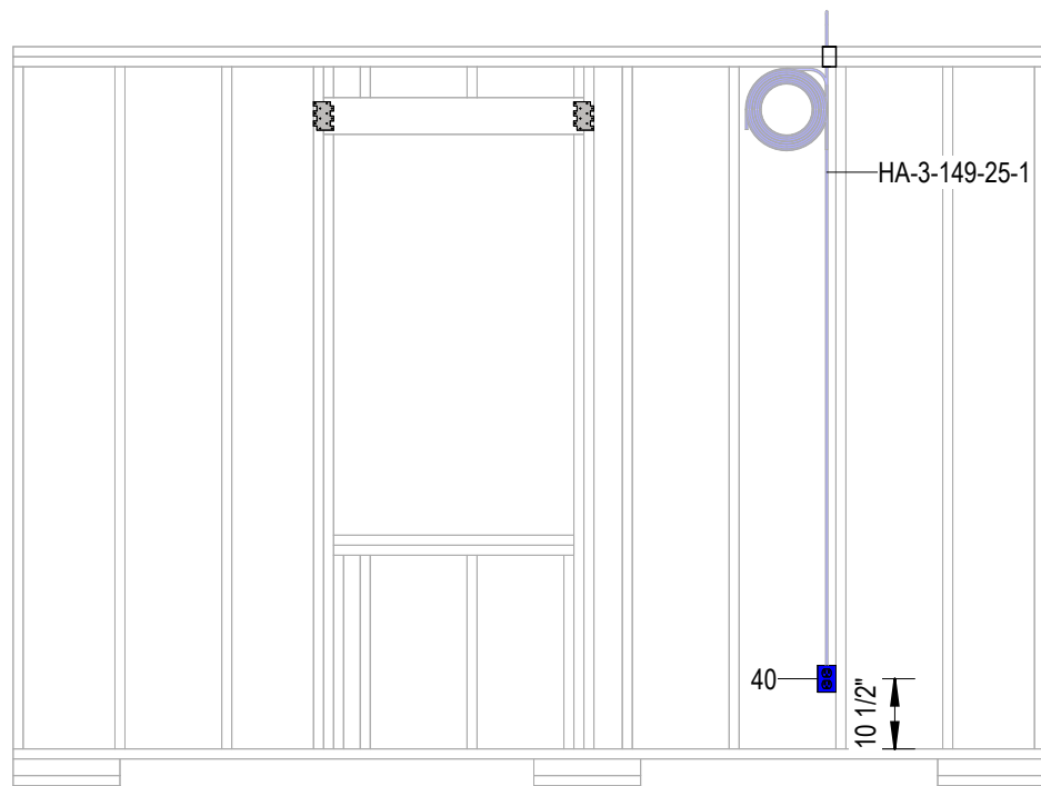
2 Electrical Side B 3/8" = 1'-0"
