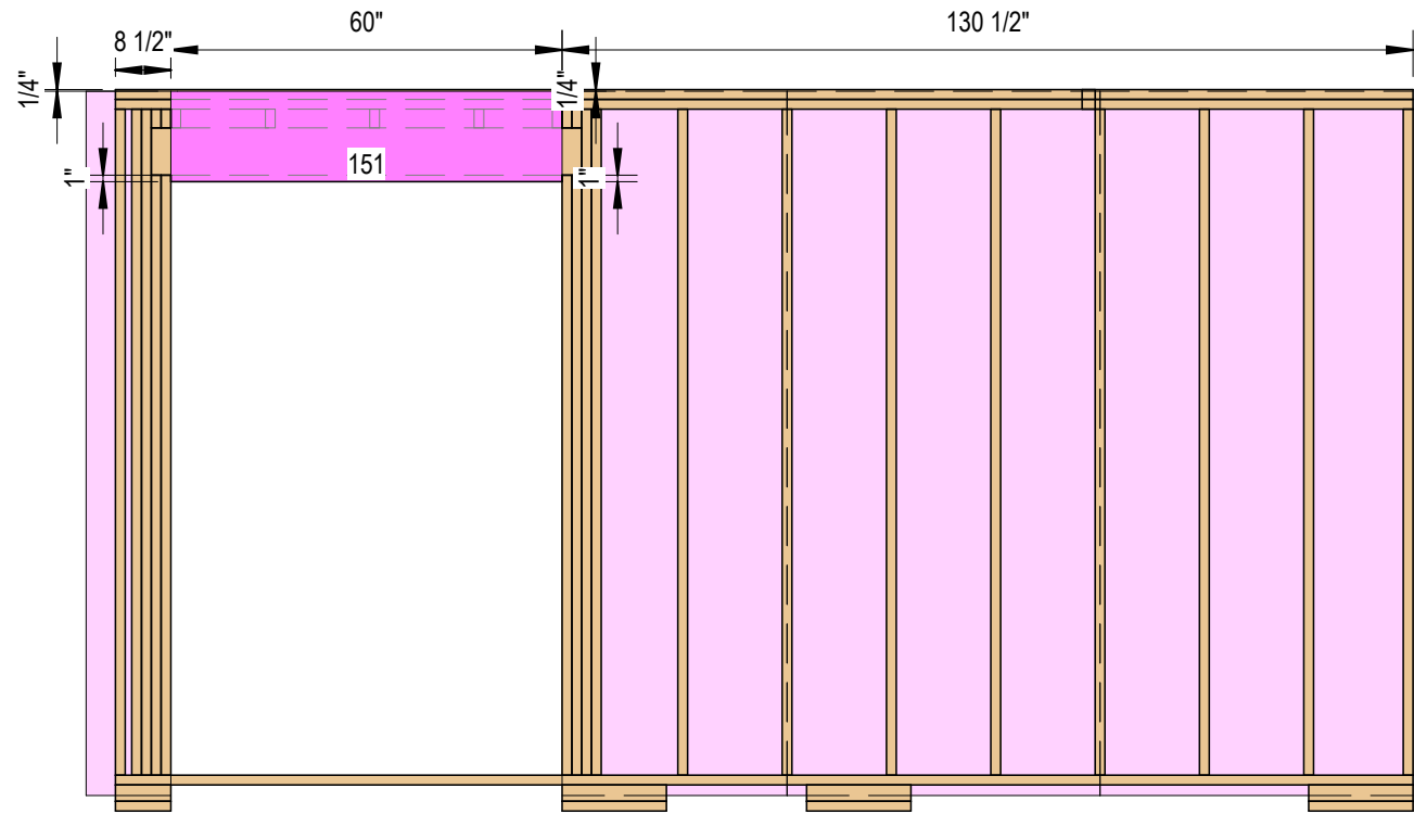
2 Sheathing Side B 3/8" = 1'-0"
