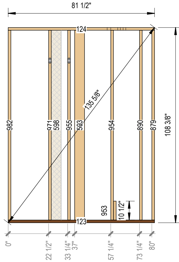
2 Framing Side A 3/8" = 1'-0"
