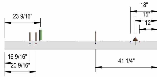
1 Top Plumbing View 3/8" = 1'-0"
